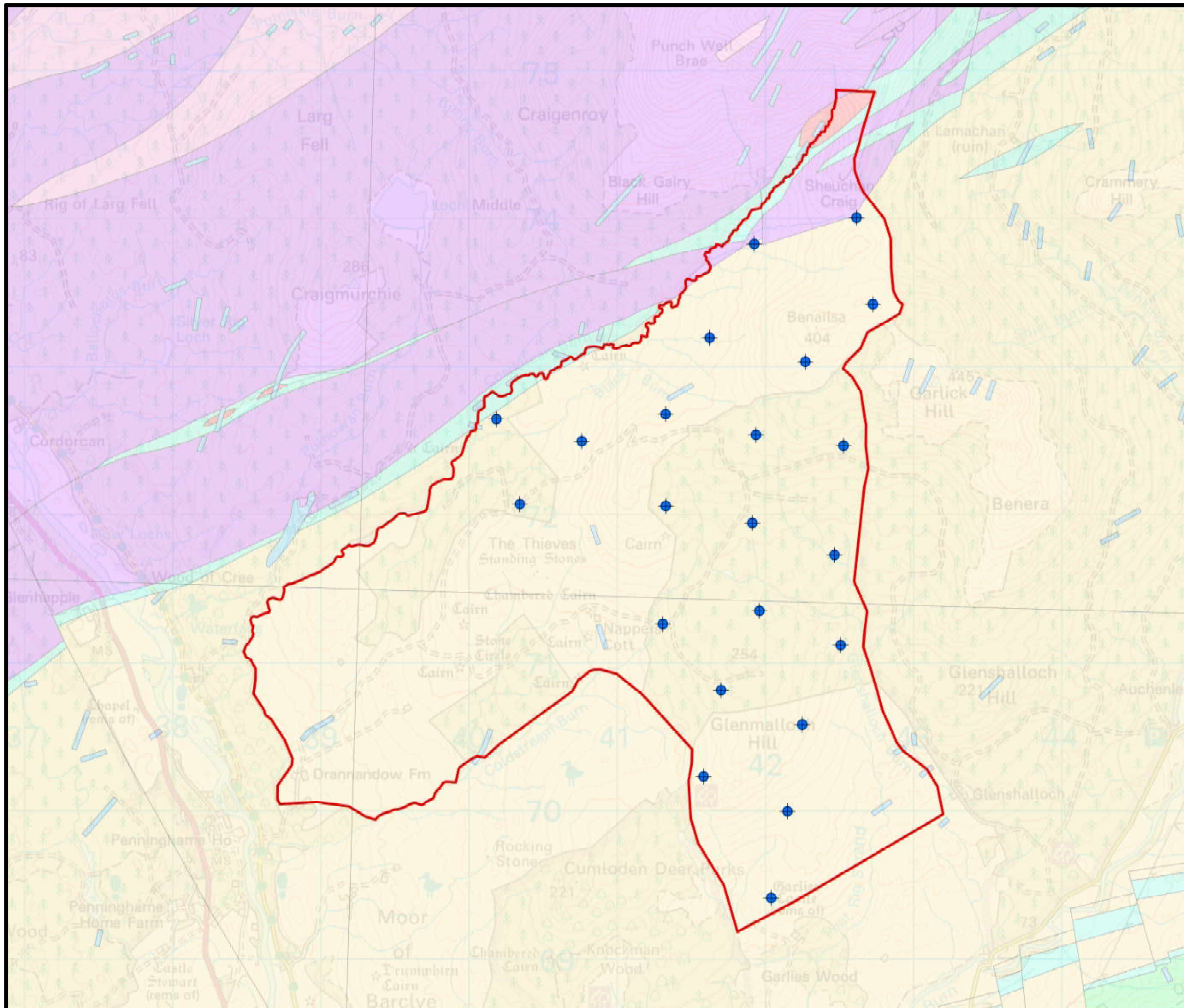
FIGURE 9.3 BEDROCK GEOLOGY
